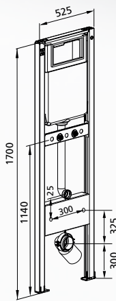
Traverse adjustable from 770-1250
