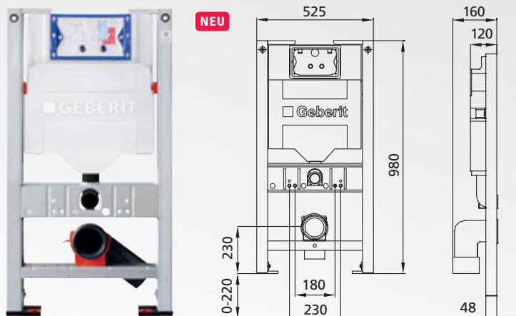
Kinder Wand-WC
