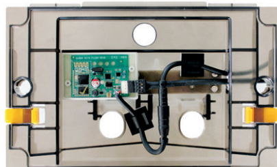
Splash protection plate incl. electronics
