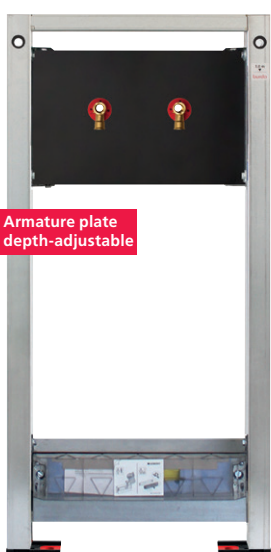
for surface-mounted fittings Installation height 1460 mm item no. 230120.00 on request also with external press connections
